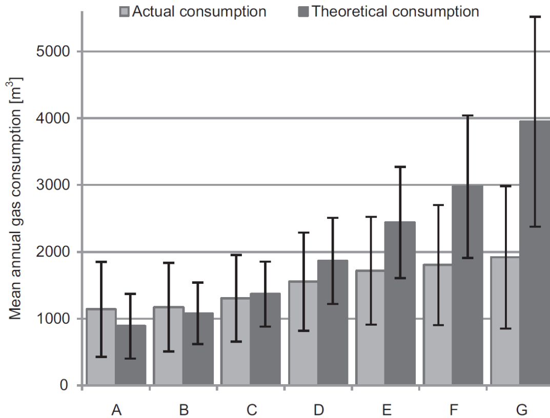
Fig. 1. Gas consumption in dwellings across label categories with \pm 1 std. deviation (Majcen et al., 2013).
